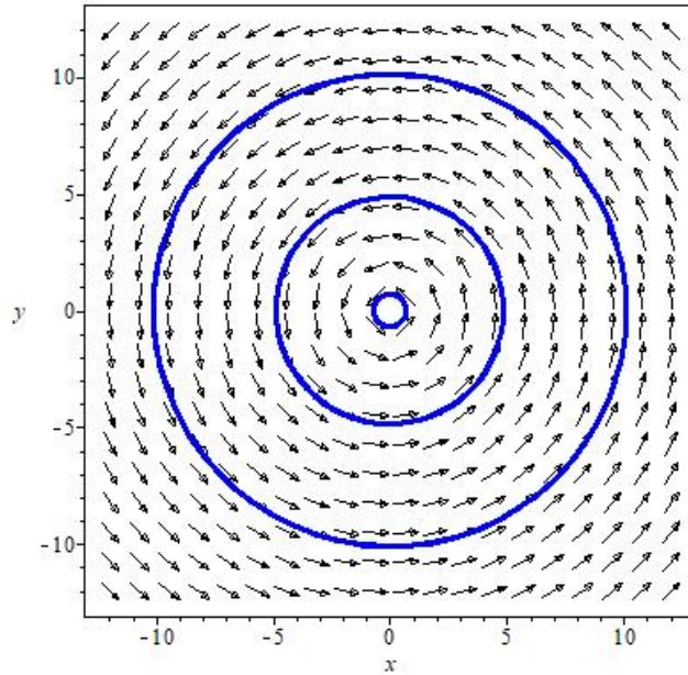
Figure 2: Three limit cycles for \varepsilon = 10^{-9} .
