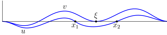
Figure 1: To Theorem 4.7.
