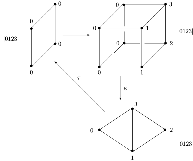
Fig. 1. The universal truncating twisting function \tau .
